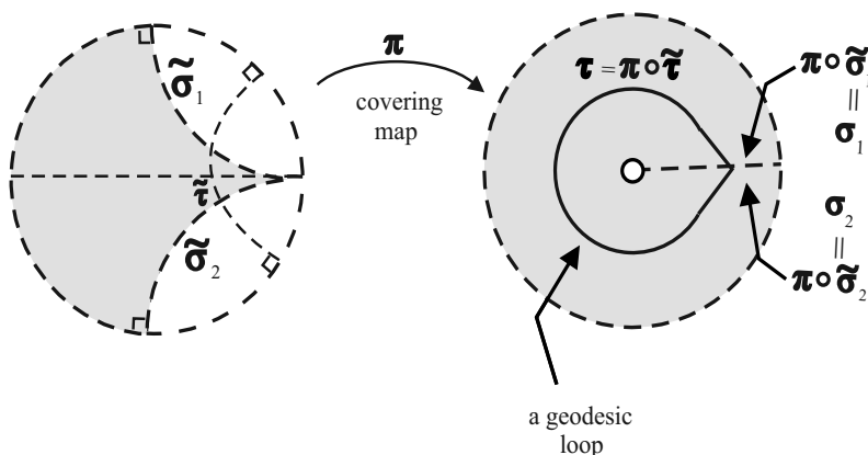
Fig. 2.3. Fundamental domain for D \rightarrow D \setminus \{0\} .
