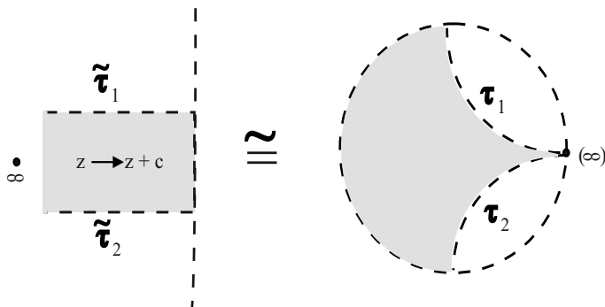
Fig. 2.4. Half-plane model vs. disc model for the covering of D \setminus \{0\} .
